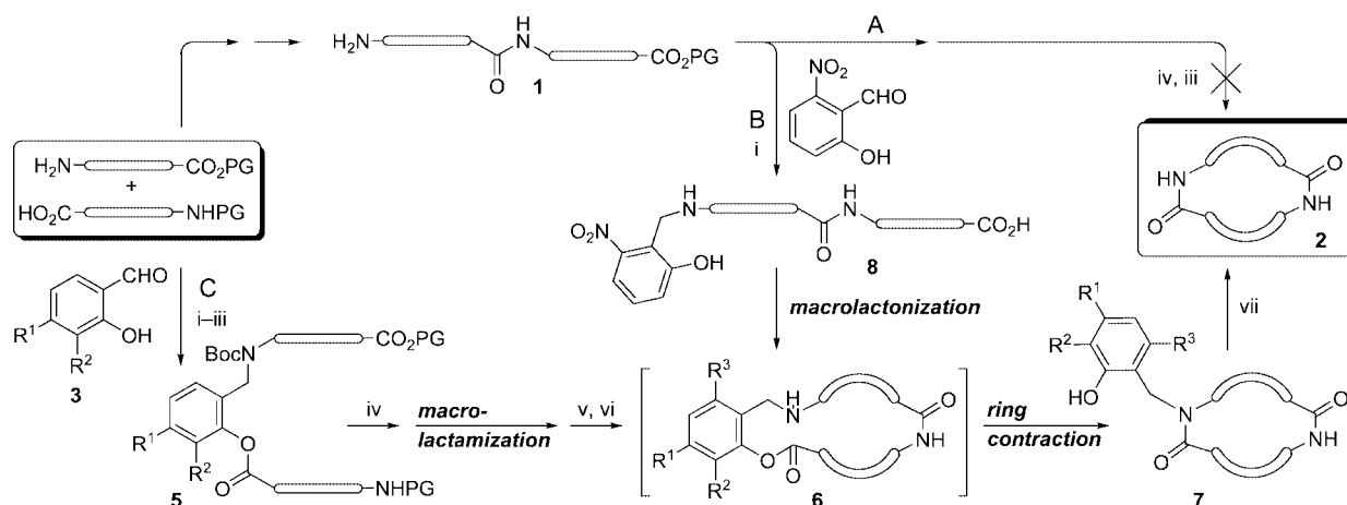
Scheme 1. General strategy for the synthesis of bis(lactams). Reaction conditions: (i) reductive amination; (ii) (Boc) 2 O; (iii) coupling reaction; (iv) protecting group removal; (v) TFA; (vi) base; (vii) auxiliary removal.
