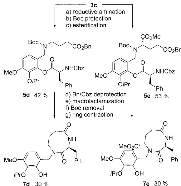
Scheme 5. Synthesis of the eight-membered bis(lactams).
