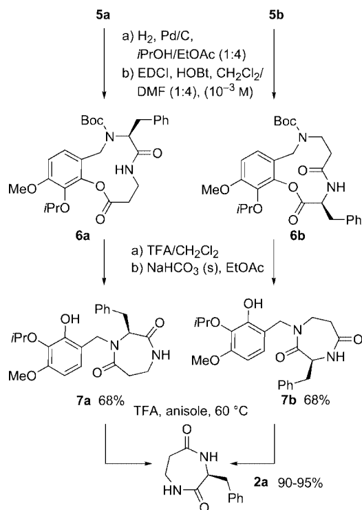
Scheme 4. Synthesis of the seven-membered bis(lactams).
