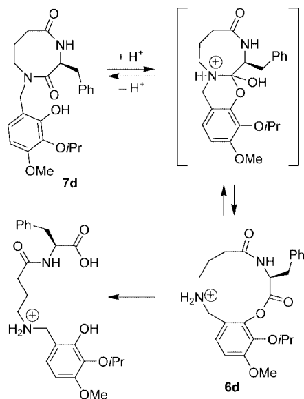
Scheme 6. Possible auxiliary-mediated side reactions from 7 .
