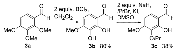
Scheme 2. Synthesis of the auxiliary.
