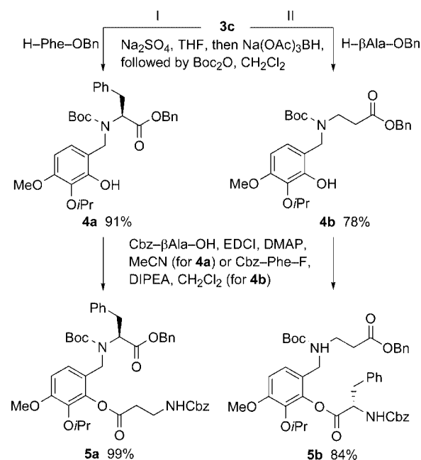
Scheme 3. Synthesis of the linear precursors.
