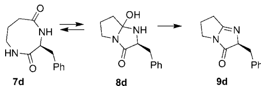
Scheme 7. Possible transannulation process providing 9d .
